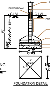
FOUNDATION DETAIL
