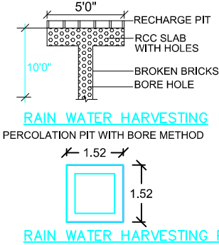
RAIN WATER HARVESTING PLAN
