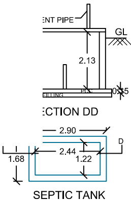
SEPTIC TANK
