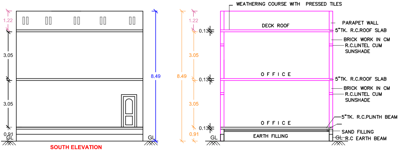
SECTION AA
