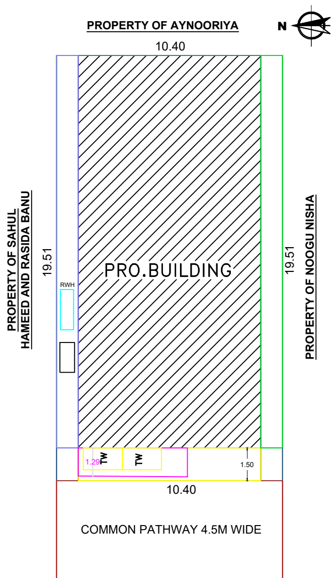
SITE PLAN
