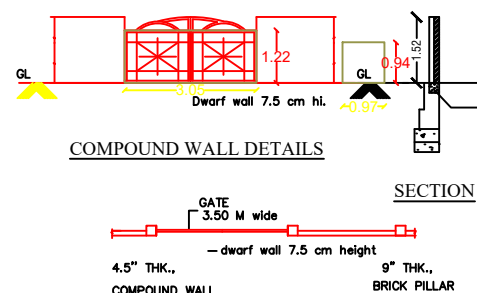
COMPOUND WALL PLAN
