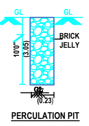
FOUNDATION DETAILS
