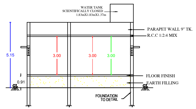
SECTION AB
