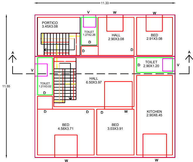
EXISTING RESIDENTIAL FIRST FLOOR APPROVAL & PROPOSED RESIDENTIAL FIRST FLOOR
