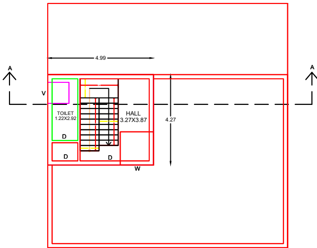
PROPOSED RESIDENTIAL SECOND FLOOR
