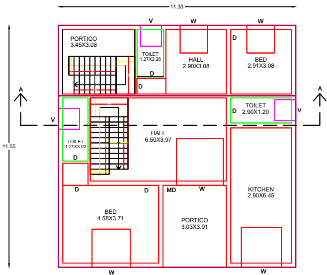
EXISTING RESIDENTIAL GROUND FLOOR APPROVAL & PROPOSED RESIDENTIAL GROUND FLOOR
