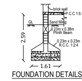
FOUNDATION DETAILS
