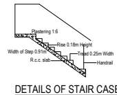
DETAILS OF STAIR CASE
