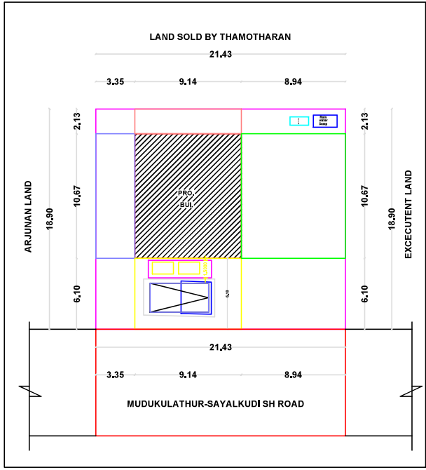
SITE PLAN & LOCATION PLAN
