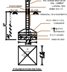
BORE WELL
