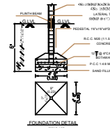
FOUNDATION DETAIL
