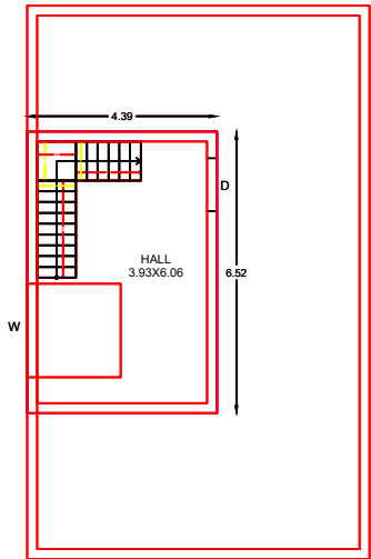
PROPOSED RESIDENTIAL FIRST FLOOR
