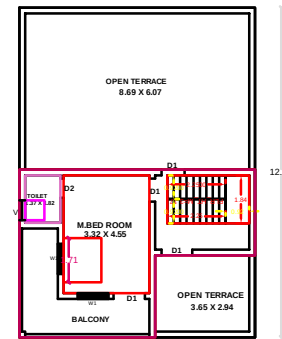
FIRST FLOOR PLAN PROPOSED
