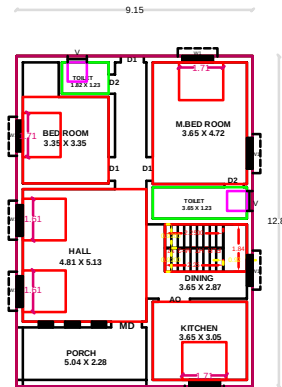
GROUND FLOOR PLAN PROPOSED
