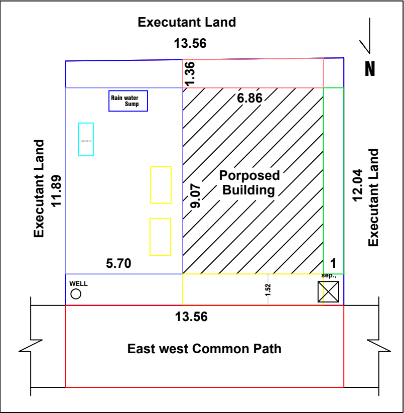
SITE PLAN CUM KEYPLAN
