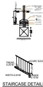
STAIRCASE DETAILS
