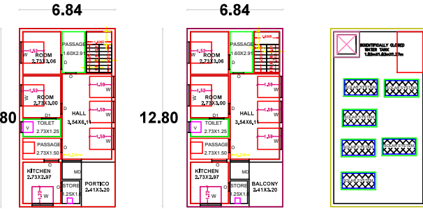
GROUND FLOOR PL
