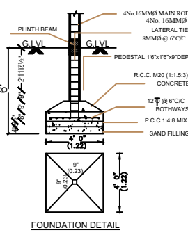
FOUNDATION DETAIL
