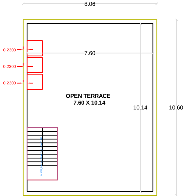
TERRACE FLOOR PLAN PROPOSED
