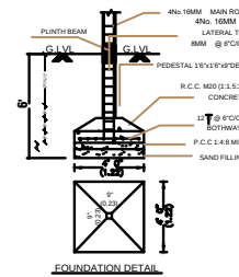
FOUNDATION DETAIL
