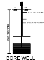
BORE WELL
