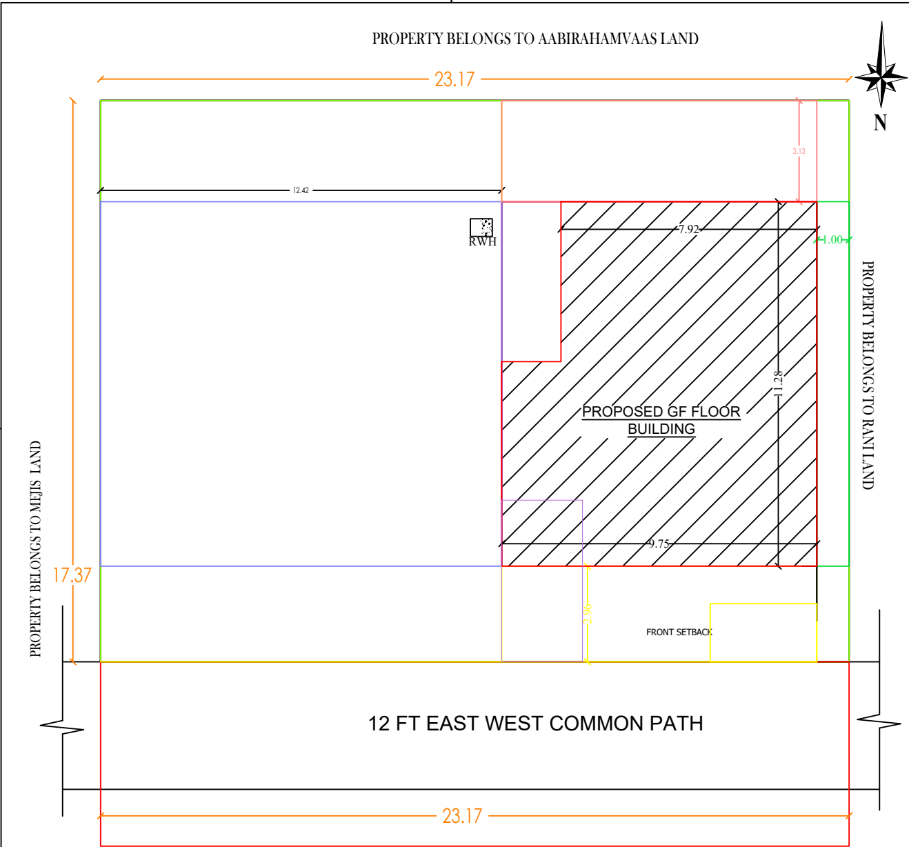
SITE PLAN
