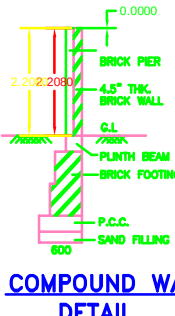
COMPOUND WALL DETAIL
