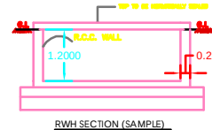
RWH_SECTION (SAMPLE)
