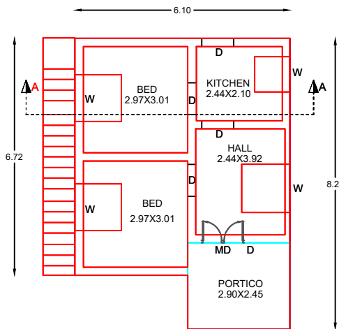
PROPOSED RESIDENTIAL GROUND FLOOR
