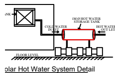
Solar Hot Water System Detail
