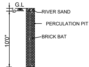
PERCULATION PIT
