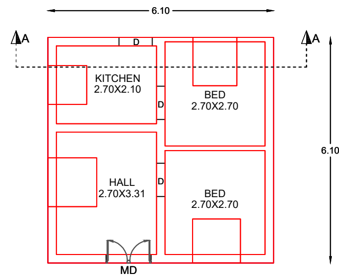
PROPOSED RESIDENTIAL GROUND FLOOR
