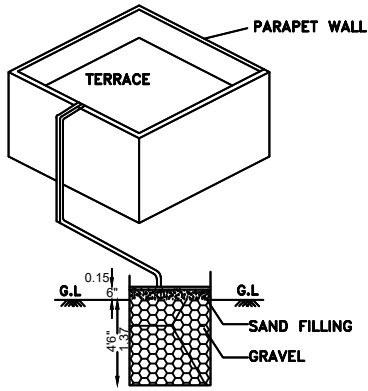
COLLECTION OF SUMP RAINWATER HARVEESTING FROM TERRACE
