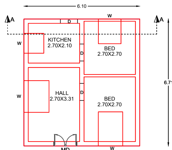
PROPOSED RESIDENTIAL GROUND FLOOR
