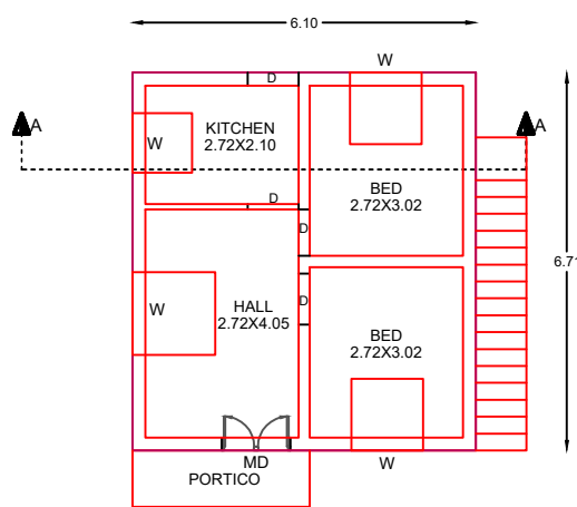
PROPOSED RESIDENTIAL GROUND FLOOR
