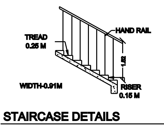
STAIRCASE DETAILS
