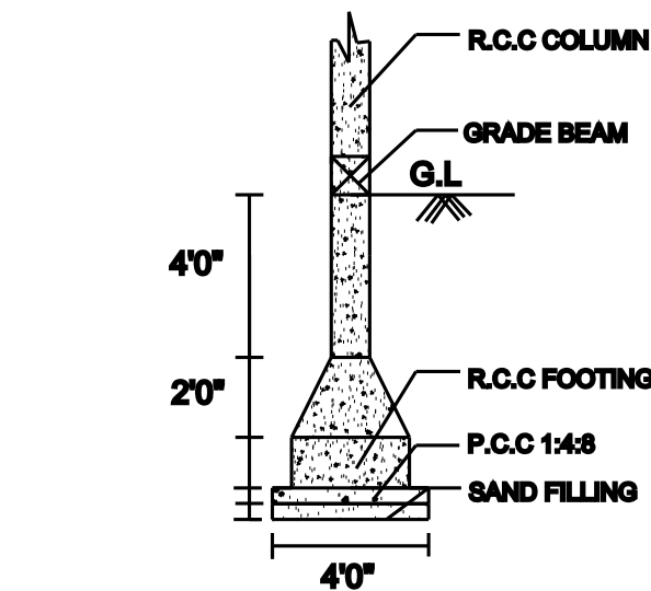
COLOUMN FOUNDATION
