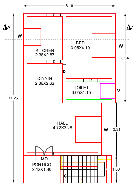
PROPOSED RESIDENTIAL GROUND FLOOR PLAN
