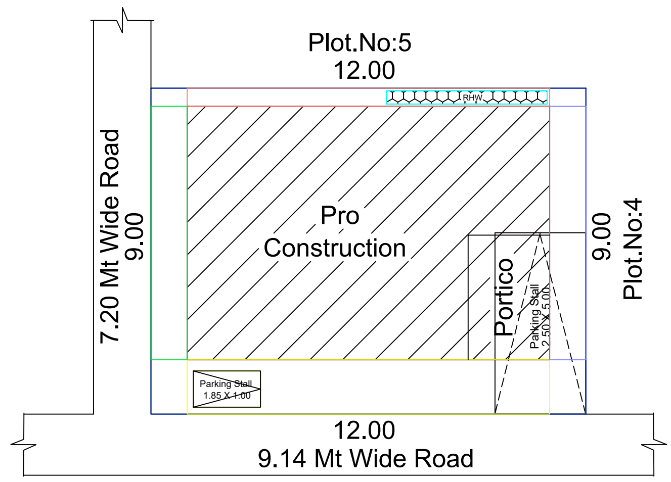
Site Plan(NTS)
