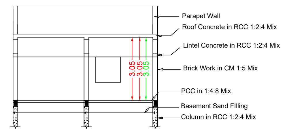
Section RR
