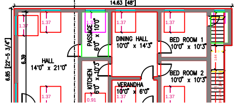
PROPOSED FIRST FLOOR
