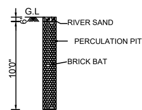
PERCULATION PIT
