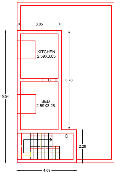
PROPOSED RESIDENTIAL FIRST FLOOR
