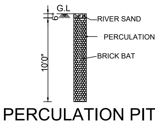
PERCOLATION PIT
