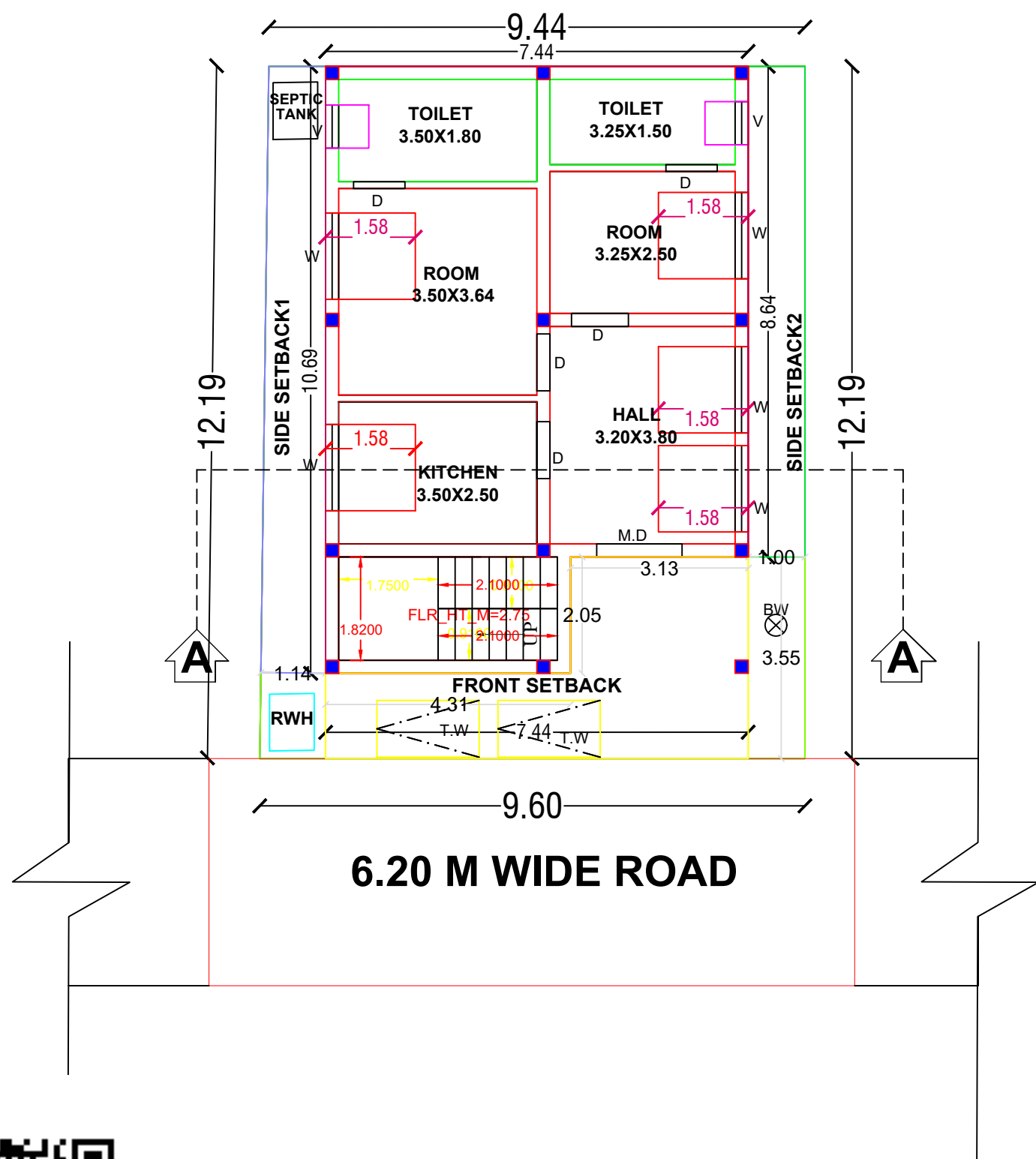
GROUND FLOOR
