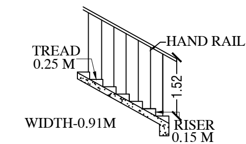
STAIRCASE DETAILS
