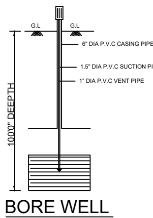
BORE WELL
