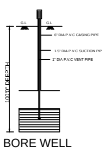
BORE WELL
