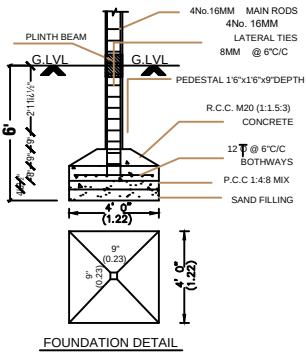
FOUNDATION DETAIL
