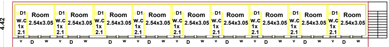
PROPOSED FIRST FLOOR PLAN
