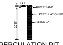
PERCOLATION PIT
