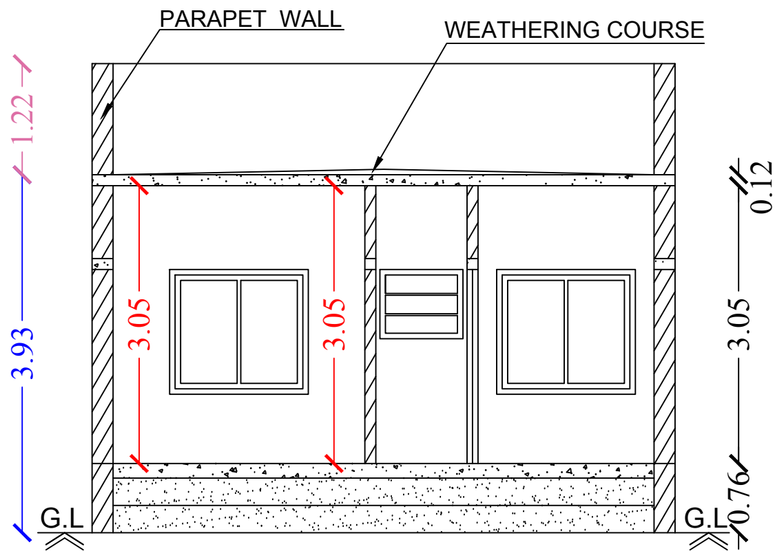
Section on-"AA"
