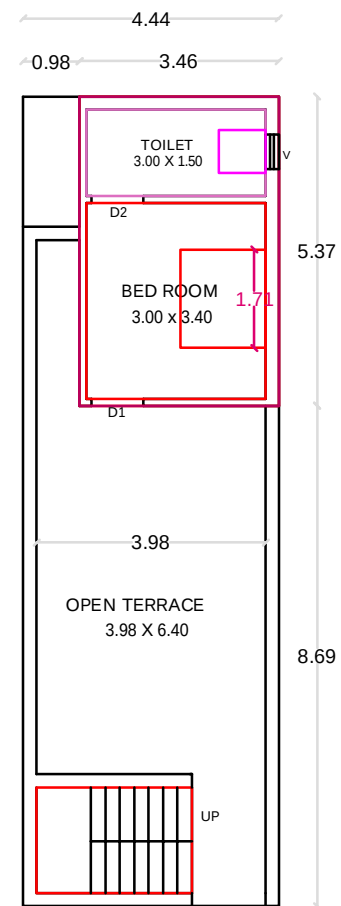
FIRST FLOOR PLAN PROPOSED
