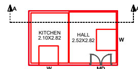
PROPOSED RESIDENTIAL GROUND FLOOR PLAN
