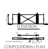
COMPOUND WALL PLAN
