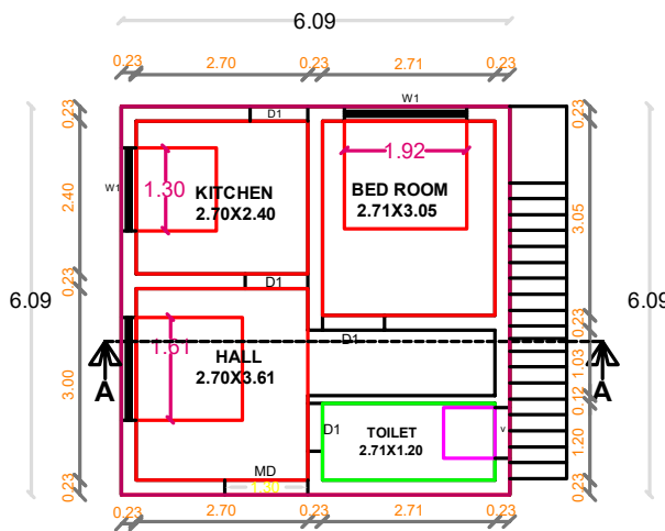
GROUND FLOOR PLAN PROPOSED
