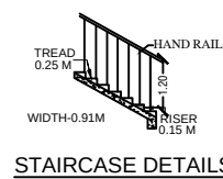
STAIRCASE DETAILS
