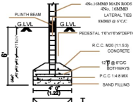
FOUNDATION DETAIL (SCALE: 1:10)
