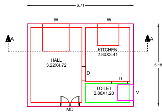
PROPOSED RESIDENTIAL GROUND FLOOR
