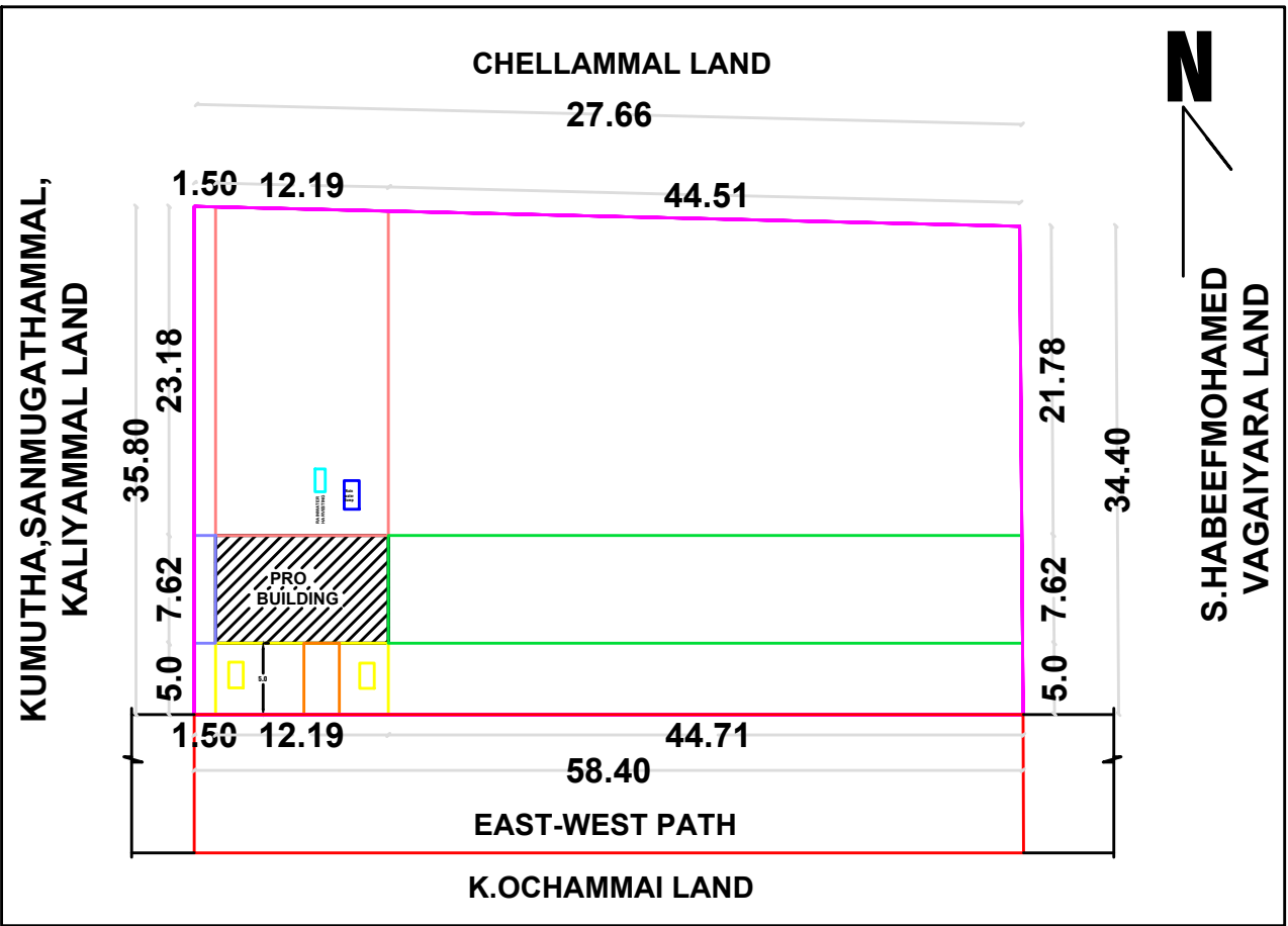
SITE PLAN & KEY PLAN (1:100)
