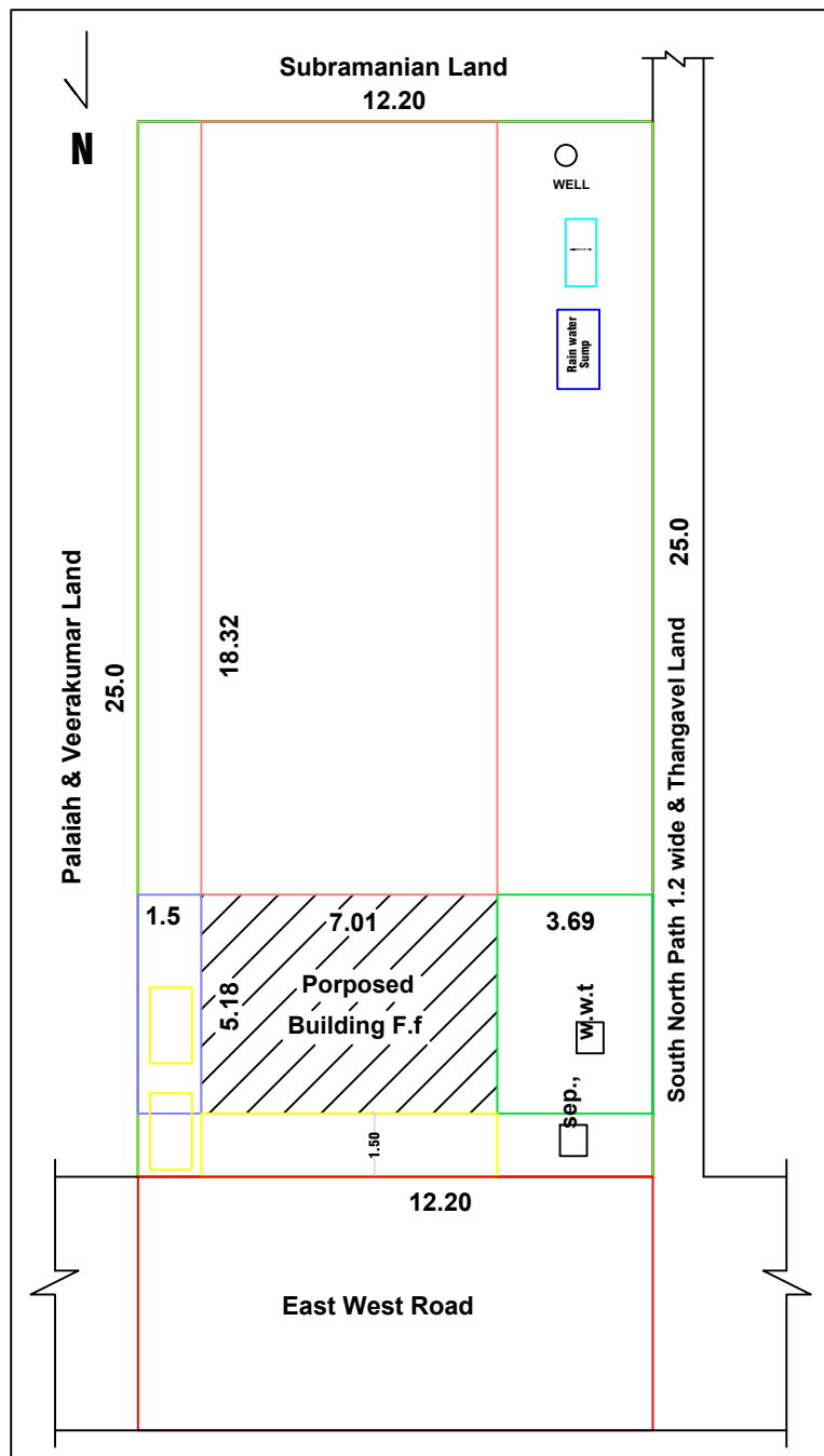
SITE PLAN CUM KEYPLAN
