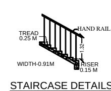
STAIRCASE DETAILS
