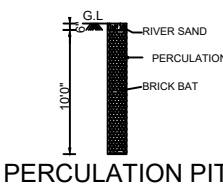
PERCOLATION PIT
