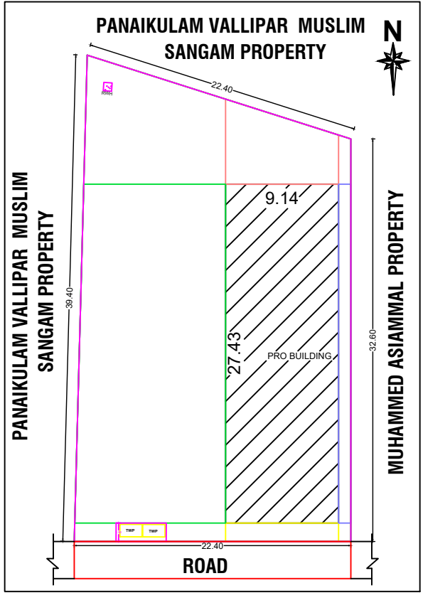
SITE PLAN
