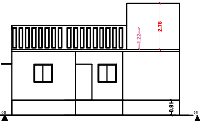
FRONT ELEVATION
