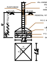
FOUNDATION DETAIL
