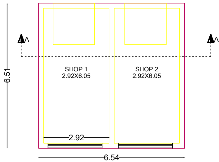
PROPOSED COMMERCIAL GROUND FLOOR PLAN
