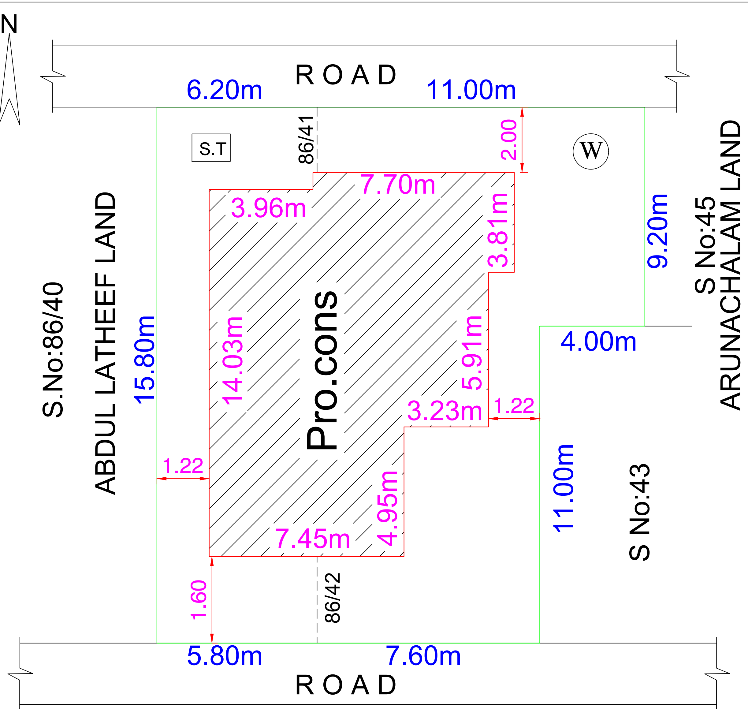
SITE PLAN
