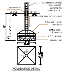
FOUNDATION DETAIL
