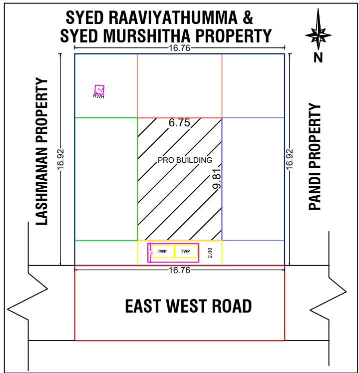
SITE PLAN
