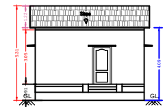
FRONT ELEVATION
